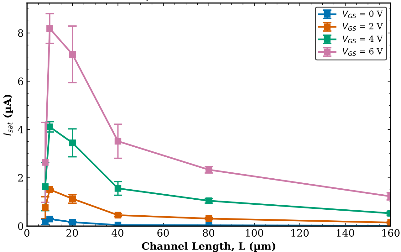
TFT1 Combined (Tr. 1 & 2) I_{sat} vs L | W = 10 \mu\text{m} (mean \pm std)
